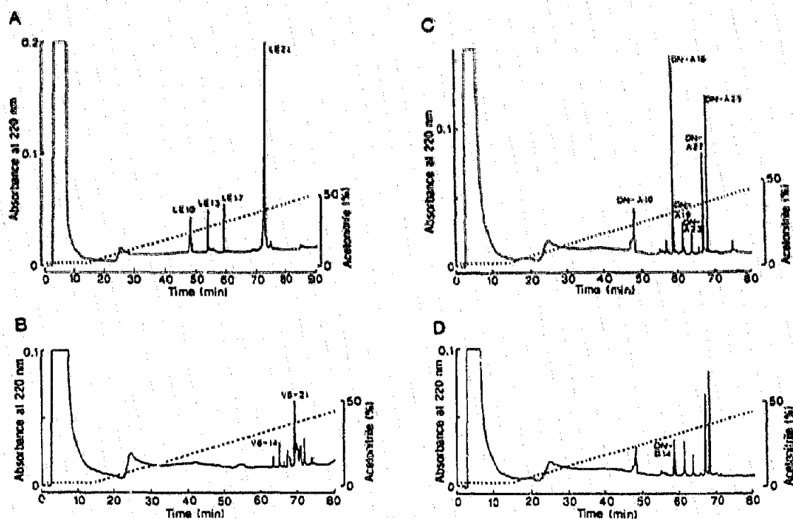
Fig. 2. Reverse-phase HPLC of enzymatic digests of dogfish CNP-115 on a Tosoh ODS-120T column. Dotted line represents a gradient of \text{CH}_3\text{CN} in 0.1% TFA. (A) Digest of CNP-115 with lysyl endopeptidase. (B) Digest of CNP-115 with Staphylococcus aureus V8 protease. (C) Digest of CNP-115 with endoprotease Asp-N. (D) Digest of LE 24 with endoprotease Asp-N.
